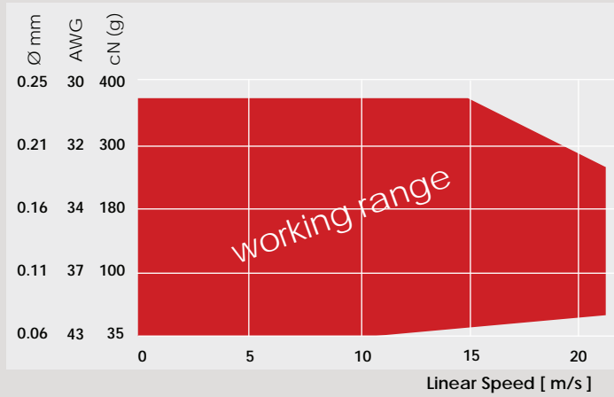
Wire / Tension
